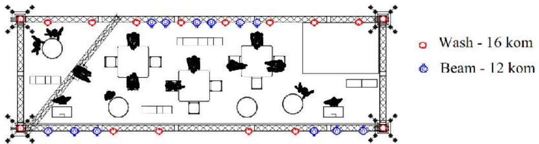
Light plot
